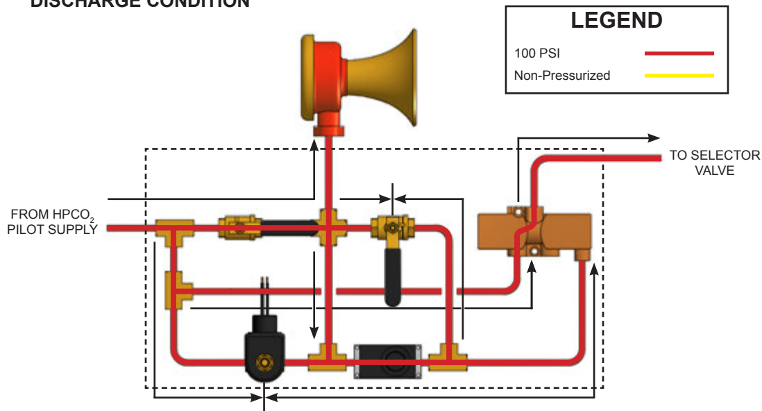
Manually Actuated Cabinet (Discharge)
