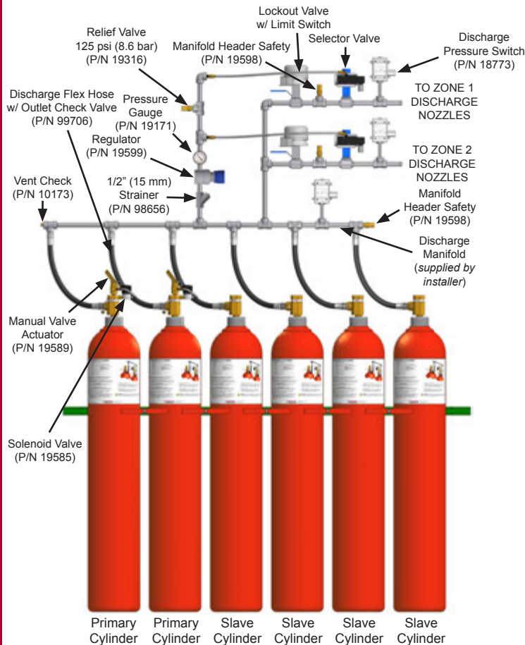
Typical Selector Valve Cylinder Arrangement
