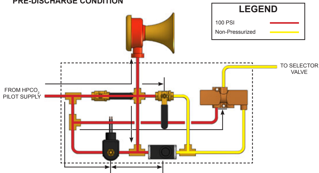
Manually Actuated Cabinet (Pre-Discharge)
