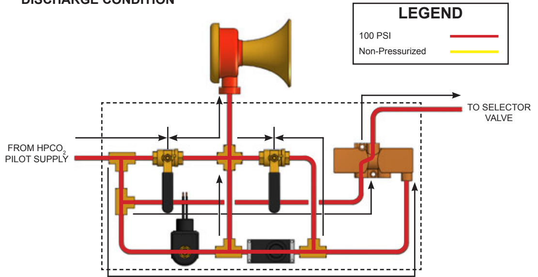
Electrically Actuated Cabinet (Discharge)
