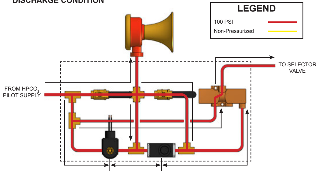
Manually Actuated Cabinet (Timer Bypass)
