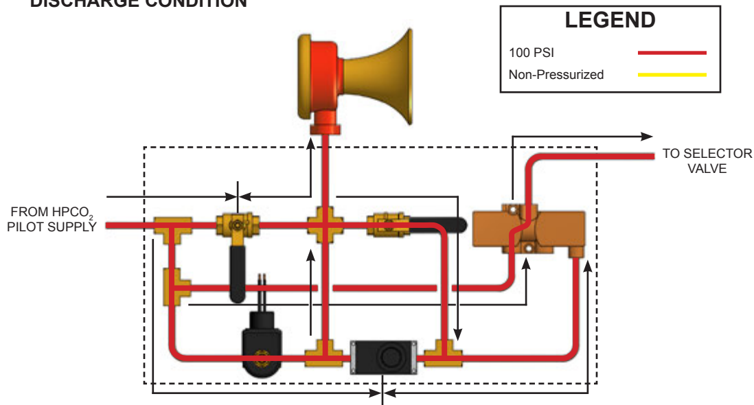
Electrically Actuated Cabinet (Timer Bypass)
