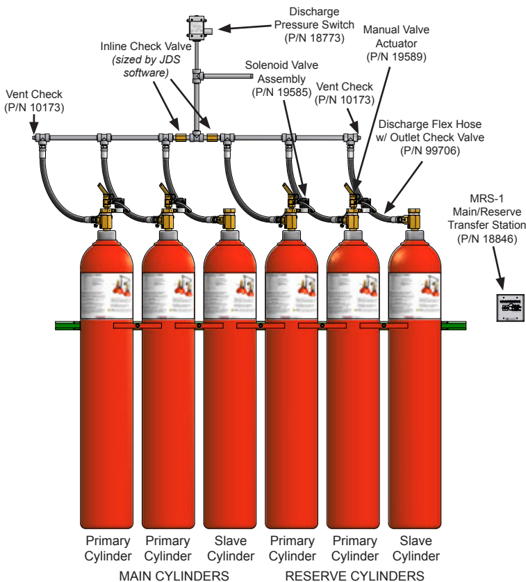
Typical Main/Reserve Cylinder Arrangement
