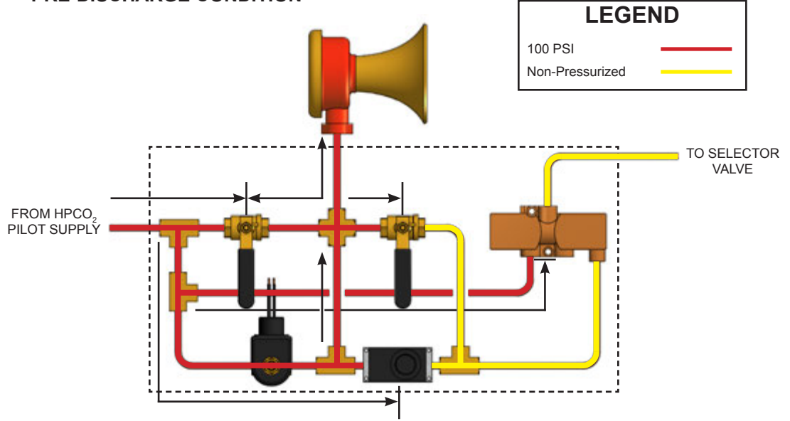
Electrically Actuated Cabinet (Pre-Discharge)
