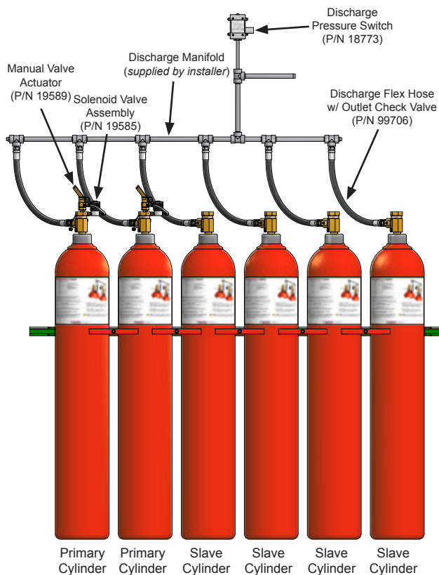
Typical Primary and Slave Cylinder Arrangement
