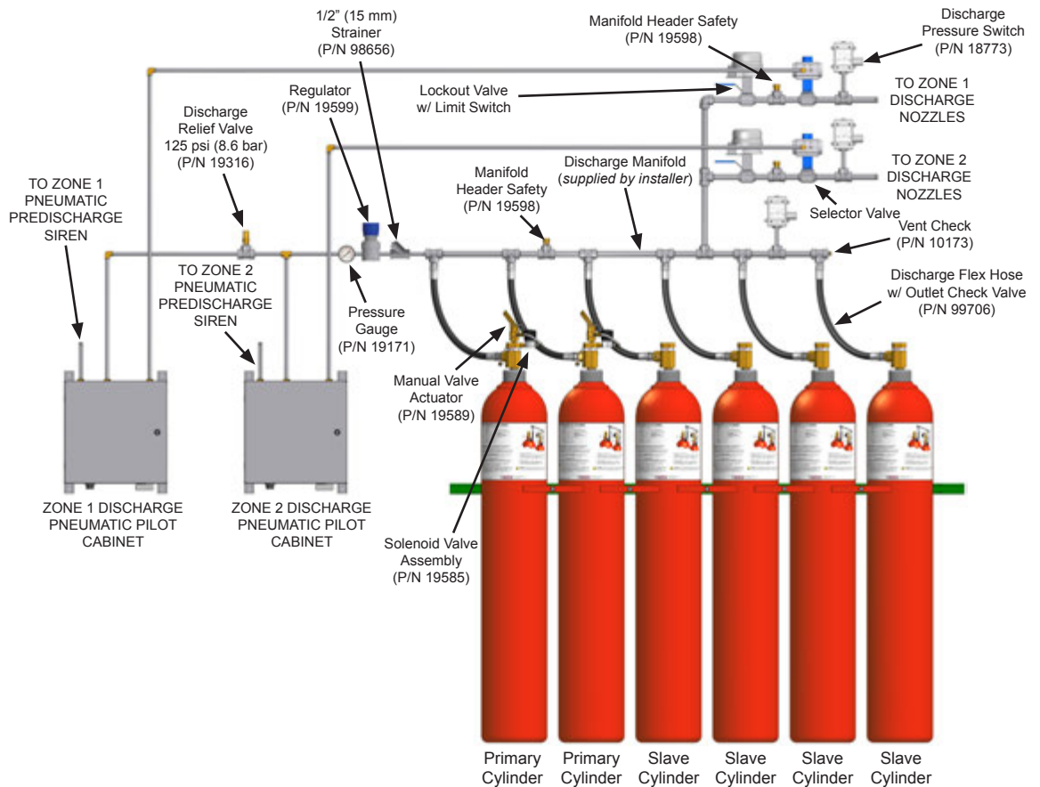
Typical Selector Valve Cylinder Arrangement w/ Pneumatic Time Delay
